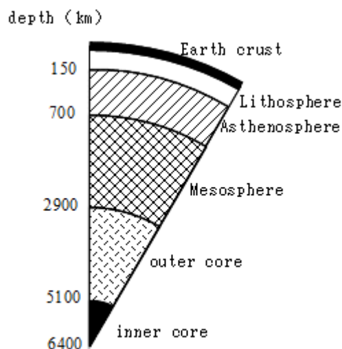
Figure A: Inside of the Earth
